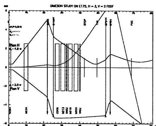
Fig. 7. Halo from splitter in standard optics.
