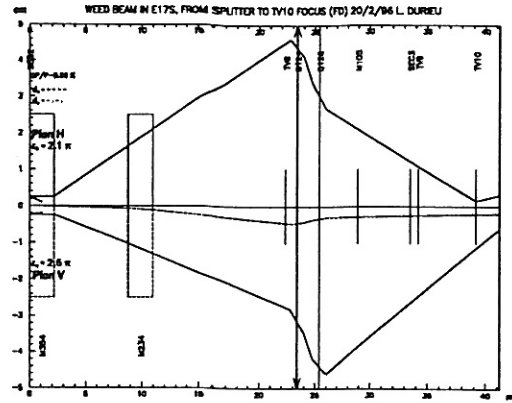
Fig. 11. Halo from splitter to TV10, optics FD.
